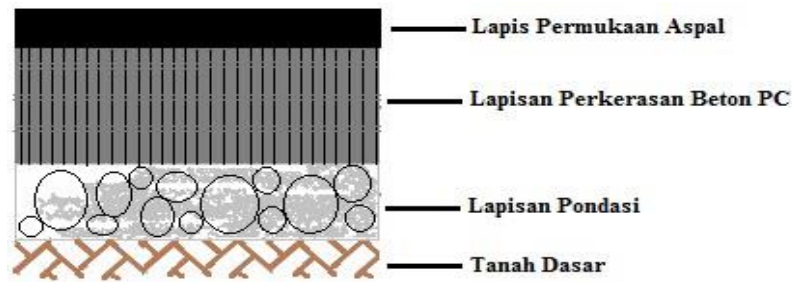
Gambar 2.3 Lapis rigid pavement
