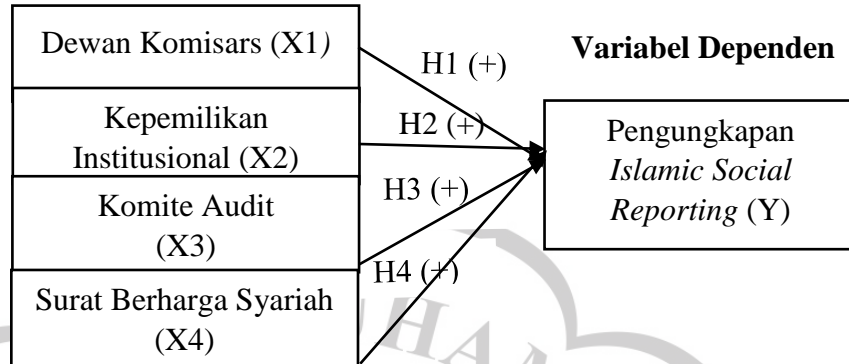
Gambar 2.1. Metode Penelitian
